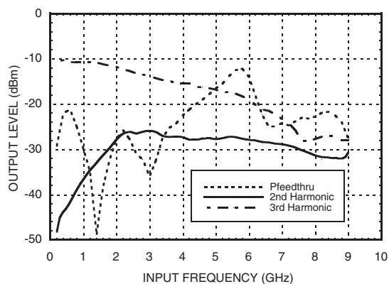
Output Harmonic
